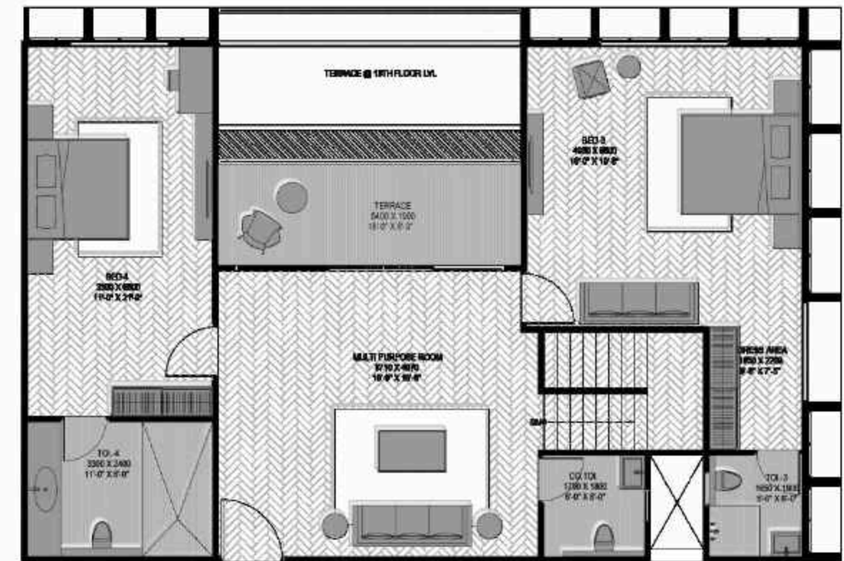
14 TH FLOOR [UPPER PENTHOUSE]
