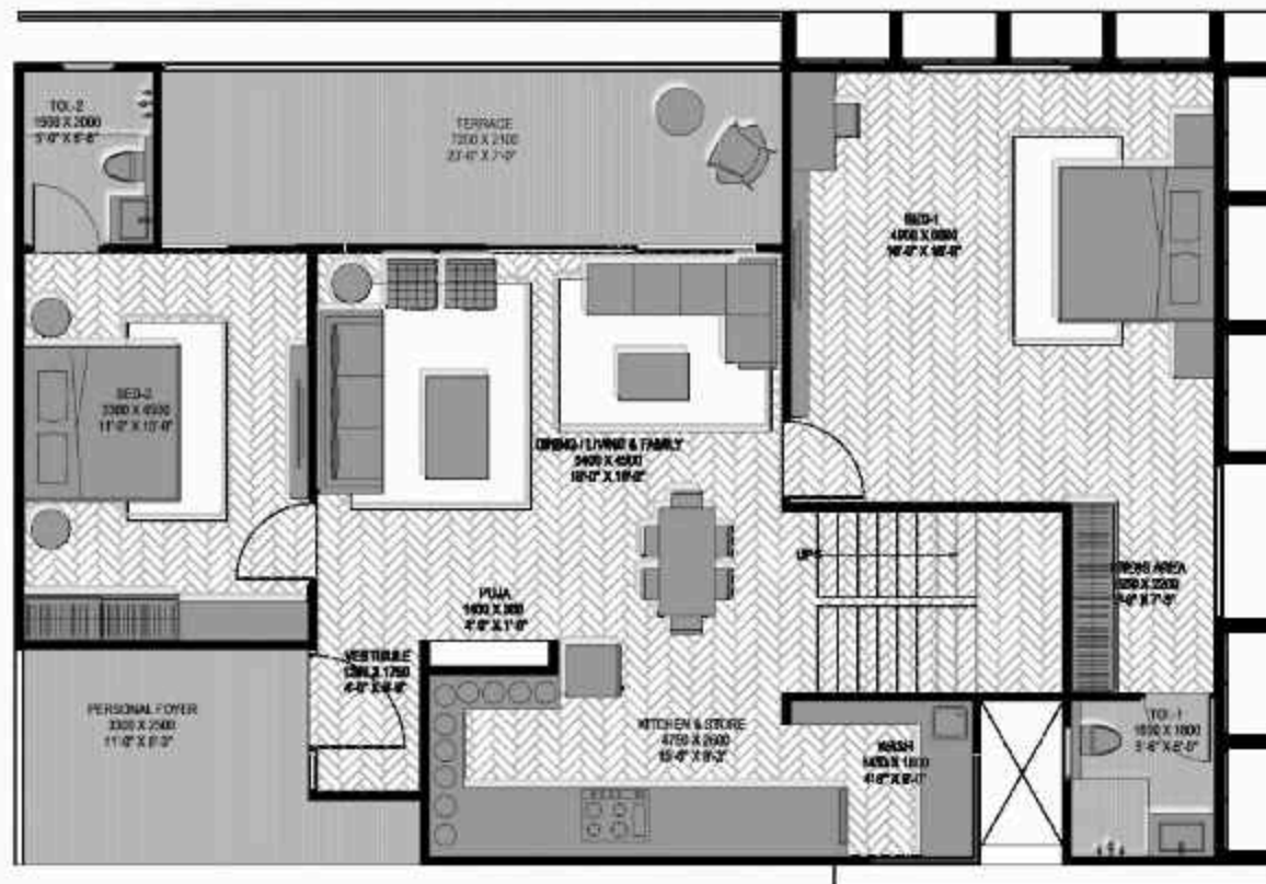
13 TH FLOOR (LOWER PENTHOUSE)
