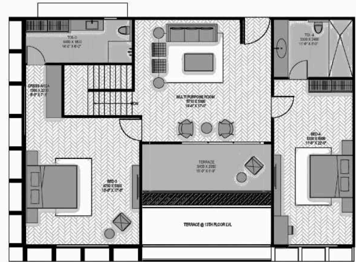
14 TH FLOOR (UPPER PENTHOUSE)
